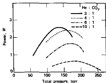
FIGURE 10.21b Output power versus total pressure under optimum pumping for \text{He}:\text{CO}_2 mixtures. Source: Reference 17.
