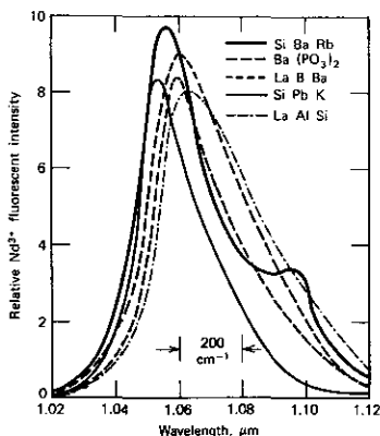
FIGURE 10.12 Fluorescent emission of the 1.06\text{ }\mu\text{m} line of \text{Nd}^{3+} at 300^\circ\text{K} in various glass bases. Source: Reference 8.
