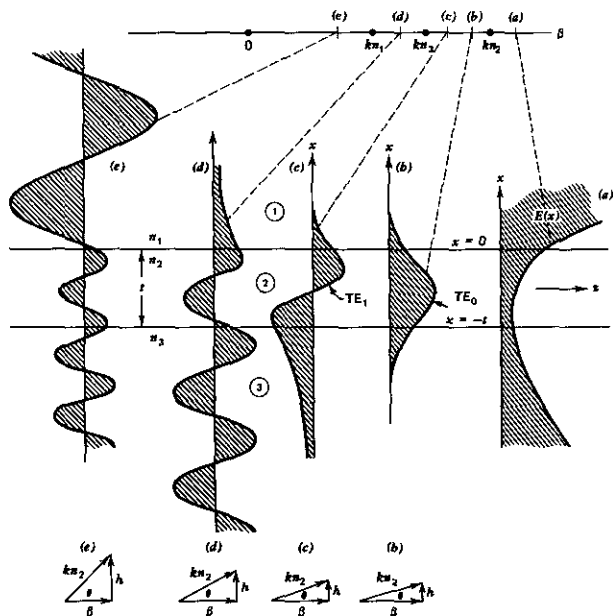
FIGURE 22.2 Top: the different regimes a , b , c , d , e of the propagation constant \beta of the waveguide shown in Figure 22.1. Middle: the field distributions corresponding to the different value of \beta . Bottom: the propagation triangles corresponding to the different propagation regimes.
