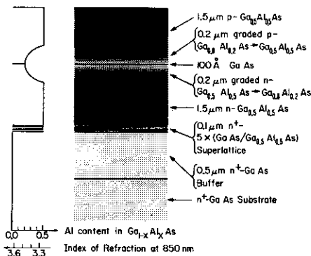
FIGURE 12.5 The actual layered structure grown by molecular beam epitaxy used to fabricate QW lasers. Source: Courtesy M. Mittelstein, L. Anders and P. Derry, California Institute of Technology, Pasadena, Calif.
