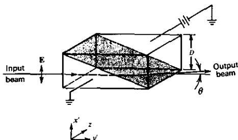
FIGURE 14.14 Double-prism KDP beam deflector. Upper and lower prisms have their z axes reversed with respect to each other. The deflection field is applied parallel to z .
