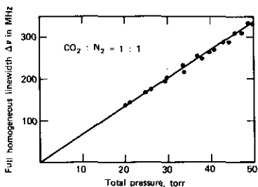
FIGURE 10.21a The 10.6\text{ }\mu\text{m} transition linewidth versus pressure for a gas mixture with equal partial pressures of \text{CO}_2 and \text{N}_2 .
