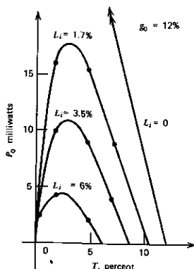
FIGURE 9.5 Useful power output ( P_0 ) versus mirror transmission T for various values of internal loss L_i in an He-Ne 6328 Å laser. Source: Reference 8.
