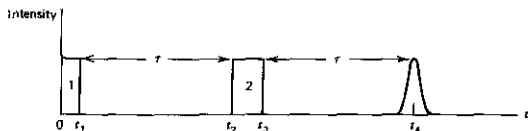
FIGURE 15.8 A \pi/2 pulse ① and a \pi pulse ② applied to an ensemble of absorbing atoms exciting a radiated echo pulse at t_4 .
