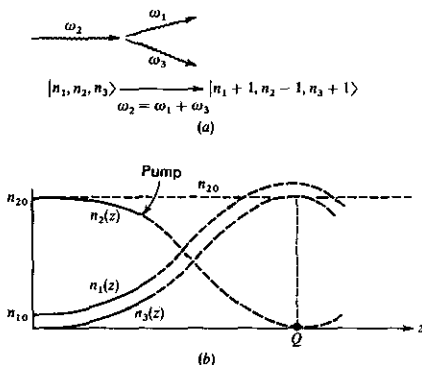
FIGURE 17.12 Parametric amplification. Here, we have energy conversion from \omega_2 to \omega_1 and \omega_3 where \omega_2 = \omega_1 + \omega_3 . The photons' densities are shown in (b). The dark portions of the curves correspond to the "nondepleted" pump approximation as described by the parametric amplification analysis of Section 17.2 (with \omega_2 taken as pump instead of \omega_3 ). The dashed curves are in the nonlinear region.
