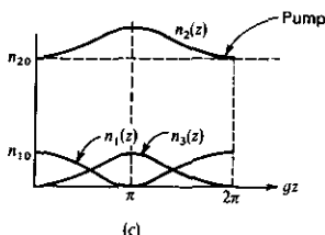
FIGURE 17.10 The process of difference frequency generation where a pump input at \omega_2 and a signal at \omega_1 > \omega_2 initially produce photons at \omega_3 = \omega_1 - \omega_2 . The process is reversed further along in the interaction path. The direction of power flow is given in (a) and (b). The photon densities are shown in (c).
