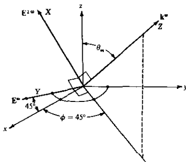
FIGURE 16.6 Second-harmonic generation in KDP. E^\omega is at 45^\circ to the x - y axes. The direction of propagation k^\omega is at angle \theta_m to the optic ( z ) axis. (All vectors passing through the dotted arc are in the x - y plane.) The effective d_{\text{eff}} is thus d_{xy} = d_{36} \sin \theta_m [see (16.5-16)].
