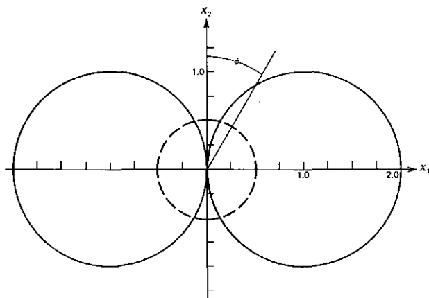
FIGURE 17.19 The rms current as a function of LO phase \phi . The dashed line is for a vacuum state ( st_I = 0 ), and the solid line is for a squeezed vacuum state ( st_I = \ln 4 ).
