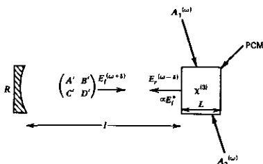
FIGURE 19.10 The phase-conjugate resonator (PCR). This general resonator is formed by placing some arbitrary optical components, represented collectively by an equivalent A'B'C'D' ray matrix, between a "real" mirror (of radius R ) at one end and a phase-conjugate mirror (PCM) at the other end. In the case of degenerate modes, which is considered here, \delta = 0 .
