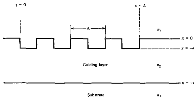
FIGURE 22.4 A corrugated periodic waveguide.
