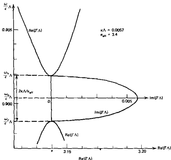
FIGURE 22.6 The dependence of the real and imaginary parts of the mode propagation constant \beta' of the modes in a periodic waveguide. At frequencies \omega_1 < \omega < \omega_2 , \text{Im}(\beta') \neq 0 and the modes are evanescent. At these frequencies, \text{Re} \beta' = \pi/\Lambda .
