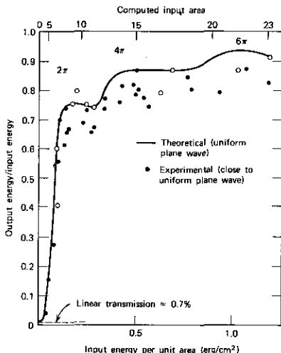
FIGURE 15.14 Self-induced transparency and nonlinear transmission in Rb vapor. Solid curve is a uniform plane-wave computer solution. Solid dots are data taken with 200\text{-}\mu\text{m} output aperture to approximate uniform plane wave. Input pulse width \sim 7 \times 10^{-9} sec. The linear low-level transmission through the cell is 0.7%. Source: Reference 14.
