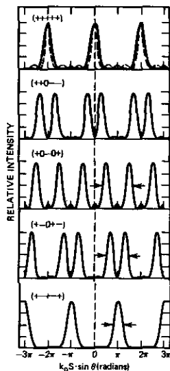
FIGURE 22.21 The grating function G for N = 5 . The dashed curve corresponds to an array of five equal amplitude ( A_i \approx 1 ) radiators. (Source: Reference 25.)
