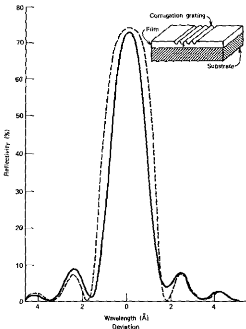
FIGURE 22.8 Illustration of corrugation filter in a thin-film waveguide, plot (solid line) of reflectivity of filter versus wavelength deviation from the Bragg condition, and calculated response of filter (dotted line) |A(0)/B(0)|^2 using (22.5-2). (Source: Reference 16).
