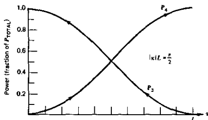
FIGURE 19.5 The intensity distribution inside the interaction region when the oscillation condition |\kappa L| = \pi/2 is satisfied.
