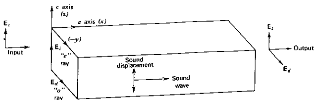
FIGURE 14.19 Collinear coupling between a z -polarized (extraordinary) and a y polarized (ordinary) optical beam by a shear S_{zx} acoustic wave.
