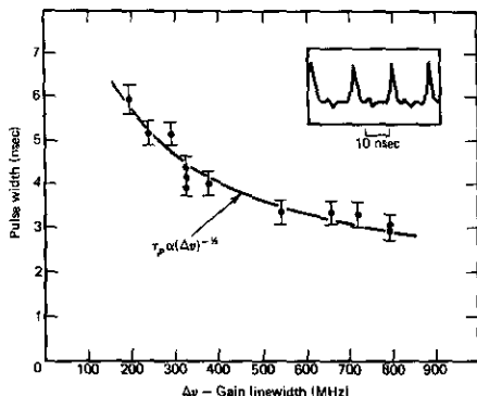
FIGURE 20.14b The dependence of the pulse width on the gain linewidth \Delta\nu that is controlled by varying the pressure ( \Delta\nu = 8 \times 10^8 at 150 torr). Source: Reference 18.
