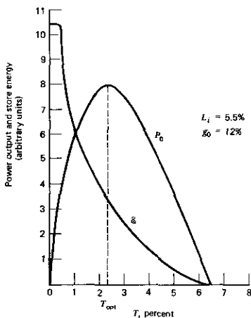
FIGURE 9.6 Power output P_0 and stored energy \mathcal{E} plotted against mirror transmission T .
