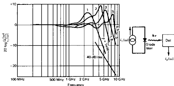
FIGURE 11.18 Modulated light output power versus current modulation frequency of a laser of length = 120 \mu\text{m} . The inset demonstrates the method of measurement. Source: Reference 18.
