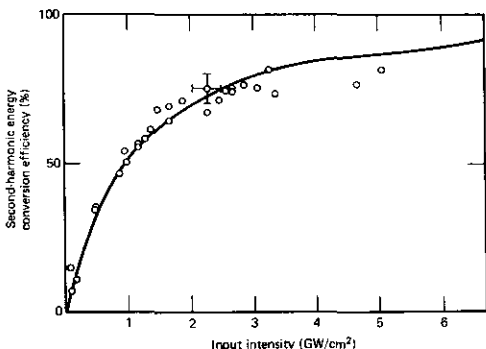
FIGURE 16.8 Frequency doubling energy conversion efficiency. Solid curve: theoretical prediction of Eq. (16.6-8) [recall that A_1(0) \propto \sqrt{I_{in}} ]. The circles correspond to experimental points. Source: Supplementary Reference 7.
