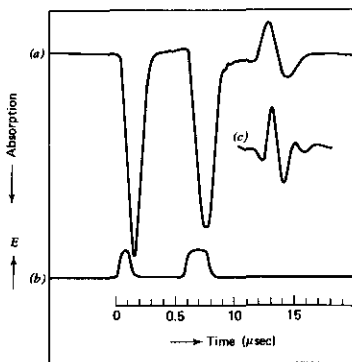
FIGURE 15.10 Photon echo in \text{C}^{13}\text{H}_3\text{F} at 5.2 m torr pressure. (a) Optical response to \pi/2 and \pi pulses followed by the photon echo. (b) The \pi/2 and \pi Stark pulses. In this experiment, the optical field was left on continuously whereas the electric field dependence of the energy levels (Stark effect) was used to switch the molecules in and out of resonance by means of the electric field pulses (b). Source: Reference 8.
