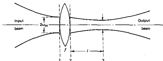
FIGURE 6.6 Focusing of a Gaussian beam.
