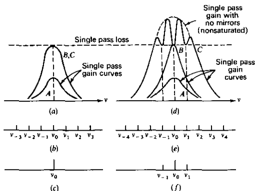
FIGURE 20.6 (a) Single-pass gain curves for a homogeneous atomic system (A—below threshold; B—at threshold; C—well above threshold). (b) Mode spectrum of optical resonator. (c) Oscillation spectrum (only one mode oscillates). (d) Single-pass gain curves for an inhomogeneous atomic system (A—below threshold; B—at threshold; C—well above threshold). (e) Mode spectrum of optical resonator. (f) Oscillation spectrum for pumping level C, showing three oscillating modes.
