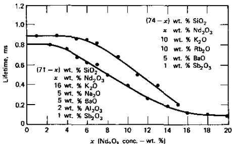
FIGURE 10.14 Lifetime as a function concentration for two glass series. Source: Reference 8.
