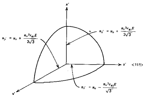
FIGURE 14.8 The intersection of the index ellipsoid of 43m crystals (with E_k parallel to \langle 111 \rangle ) with the planes x' = 0 , y' = 0 , z' = 0 . The principal indices of refraction for this case are n_{x'} , n_{y'} , and n_{z'} .
