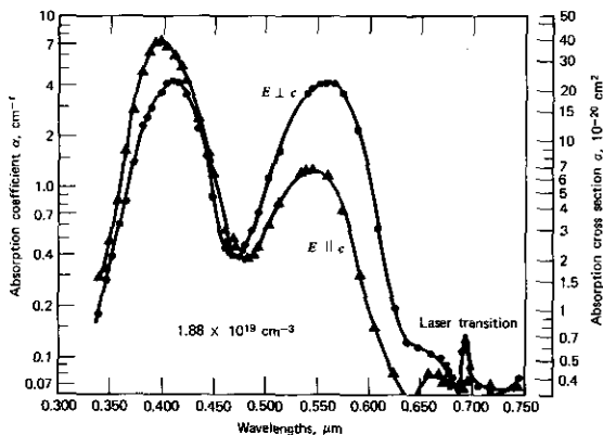
FIGURE 10.3 Absorption coefficient and absorption cross section as functions of wavelength for E \parallel c and E \perp c . The 300°K data were derived from transmittance measurements on pink ruby with an average Cr ion concentration of 1.88 \times 10^{19} \text{ cm}^{-3} . Source: Reference 3.
