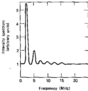
FIGURE 20.19 The intensity fluctuation spectrum of the laser output shown in Figure 20.18. Source: Reference 21.
