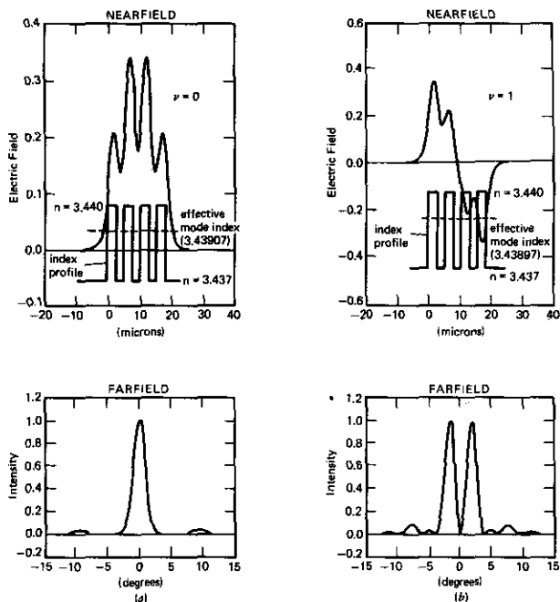
FIGURE 22.20 The four supermodes of an index-guided four-channel array. (a) The lowest-order (highest \beta ) \nu = 0 mode. (b), (c), (d) The next three modes in decreasing order of \beta . The upper figure in each case shows the near-field in relation to the channel array. The lower figure is that of the far-field. The individual channel waveguides can support a single mode (each) only. (Source: Courtesy of C. Lindsey, California Institute of Technology, Pasadena, Calif.)
