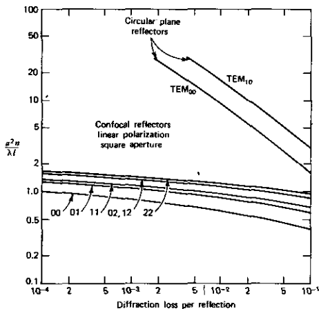
FIGURE 7.7 Diffraction losses for a plane-parallel and several low-order confocal resonators; a is the mirror radius and l is their spacing. The pairs of numbers under the arrows refer to the transverse-mode indices m, n . Source: Reference 5.
