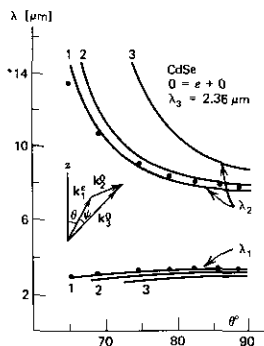
FIGURE 17.8 Angle tuning curves for CdSe with \lambda_3 = 2.36 \mu . 1 = collinear interaction \psi = 0^\circ ; 2, 3, = noncollinear interaction \psi = 0.5^\circ, 1^\circ ; \mathbf{k}_3, \mathbf{k}_1, \mathbf{k}_2 = wave vectors of pump, signal, idler frequencies; \theta = angle between signal wave vector and CdSe optic axis; \psi = angle between pumping wave vector and signal 1. Source: Reference 12.
