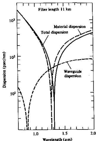
FIGURE 22.23 Pulse dispersion through a 11-km-long strand of single-mode graded-index (see Section 3.4) optical fibers. The "zero-dispersion" wavelength is 1.32\ \mu\text{m} . The material dispersion has different signs in the wavelength regions below and above its "zero-point" at 1.27\ \mu\text{m} . To obtain D in units of \text{psec}/(\text{nm}\cdot\text{km}) , we need divide the abscissa by the fiber length L = 11\ \text{km} .
