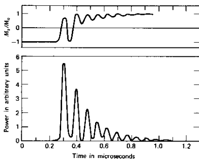
FIGURE 15.6 Superradiant emission of an inverted spin system. Upper trace: magnetization. Lower trace: radiated power. Source: Reference 5.
