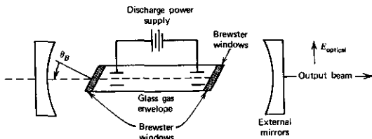
FIGURE 10.16 Typical gas laser.
