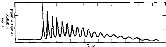
FIGURE 20.17 Intensity relaxation oscillation in a \text{CaWO}_4:\text{Nd}^{3+} laser at 1.06\text{ }\mu\text{m} . Horizontal scale = 20\text{ }\mu\text{sec/div} . Source: Reference 20.
