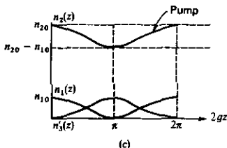
FIGURE 17.11 The process of sum frequency generation where a pump photon at \omega_2 and a signal photon at \omega_1 combine initially to generate a photon at \omega_3' = \omega_1 + \omega_2 . The process is reversed further along the interaction path. The direction of power flow is given in (a) and (b). The photon densities are drawn in (c).
