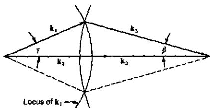
FIGURE 18.8 A construction for finding the direction of propagation k_1 of the anti-Stokes radiation.
