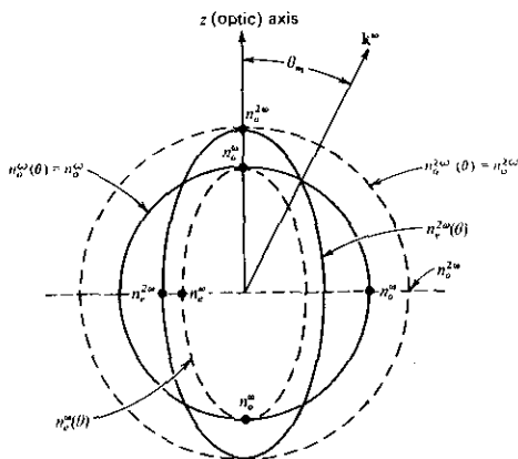
FIGURE 16.5 Normal (index) surfaces for the ordinary and extraordinary rays in a negative ( n_e < n_o ) uniaxial crystal. If n_e^{2\omega} < n_o^{2\omega} , the condition n_e^{2\omega}(\theta) = n_o^{2\omega} is satisfied at \theta = \theta_m . The eccentricities shown are exaggerated.
