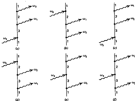
FIGURE A.4-2 The Feynman diagrams used to derive the six terms of the optical nonlinear constants d_{32}^{(2)\omega_1\omega_2} . These diagrams correspond to the six permutations of the sequence of photon interactions in a process in which an atom makes a transition |1\rangle \rightarrow |3\rangle \rightarrow |2\rangle \rightarrow |1\rangle while absorbing a photon at \omega_3 and emitting photons at \omega_1 and \omega_2 . Since \omega_3 = \omega_1 + \omega_2 , energy is conserved. The amplitudes corresponding to these diagrams are given in (A.4-19).
