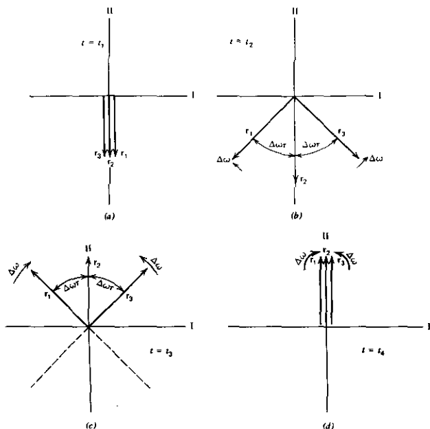
FIGURE 15.9 The atomic \mathbf{r}_a vectors at (a) t = t_1 , (b) t = t_2 , (c) t = t_3 , (d) t = t_4 .
