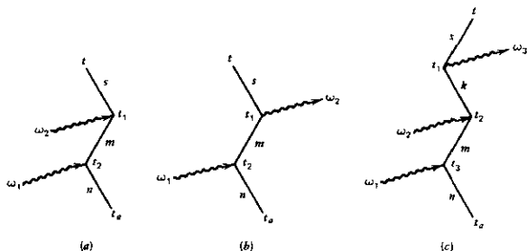
FIGURE 3.1 The Feynman diagrams used to obtain (a) \Psi_{-\omega_1, -\omega_2}^{(2)}(t) , (b) \Psi_{-\omega_1, \omega_2}^{(2)}(t) , (c) \Psi_{-\omega_1, -\omega_2, \omega_3}^{(3)}(t) .
