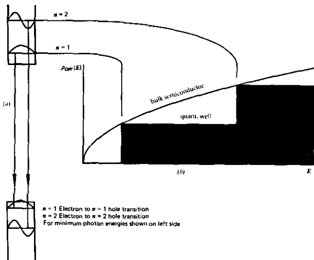
FIGURE 12.2 (a) The first two n = 1 , n = 2 quantized electron and hole states and their eigenfunctions in an infinite potential well. (b) A plot of the volumetric density of states (1/L_z)/[dN(E)/dE] (i.e., the number of states per unit area per unit energy divided by the thickness of the action region) of a quantum well and of a bulk semiconductor. Source: Courtesy of M. Mittelstein, California Institute of Technology, Pasadena, Calif.
