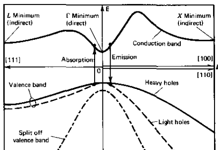
FIGURE 11.1b Plot of energy versus wave-vector for electrons in conduction and valence bands of direct-gap semiconductor, for example, GaAs (diagrammatic). Source: Reference 10.
