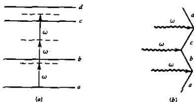
FIGURE 18.1 (a) The energy level diagram of an atom (molecule) responsible for third-harmonic generation. (b) The dominant Feynman diagram used in the calculation of \chi^{(3\omega=\omega+\omega+\omega)} .
