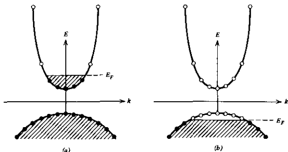
FIGURE 11.2 (a) Energy band of degenerate n type of semiconductor at 0^\circ\text{K} . (b) A degenerate p type of semiconductor at 0^\circ\text{K} . The cross hatching represents regions in which all the electron states are filled. Empty circles indicate unoccupied states.
