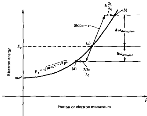
FIGURE 13.7 Dispersion diagram (similar to Figure 13.1) demonstrating why an electron (with energy E_e ) emits and absorbs photons at two different frequencies. The horizontal segments of length \hbar 2\pi/\lambda_0 represent the momentum supplied (in absorption) or taken up (in emission) by the periodic structure (wiggler) of period \lambda_0 . Since the final electron states (b) or (d) must fall on the electron dispersion curve E_e vs. p and the wiggler "momentum" 2\pi\hbar\lambda_0^{-1} is fixed, the frequencies of the photons absorbed or emitted by the electrons at (a) are uniquely determined as shown.
