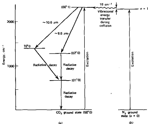
FIGURE 10.17 (a) Some of the low-lying vibrational levels of the carbon dioxide (CO 2 ) molecule, including the upper and lower levels for the 10.6 and 9.6 μm laser transitions. (b) Ground state (v = 0) and first excited state (v = 1) of the nitrogen molecule, which plays an important role in the selective excitation of the (00 1 1)CO 2 level.
