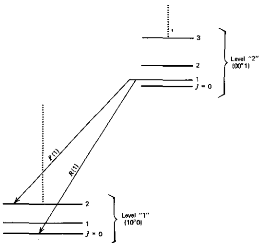
FIGURE 10.19 The vibrational-rotational level scheme of a \text{CO}_2 laser near 10.6 \mu . Transitions from J \rightarrow J + 1 are named P(J) those from J \rightarrow (J - 1) are R(J) . Only some of the low J (rotational) levels are shown.
