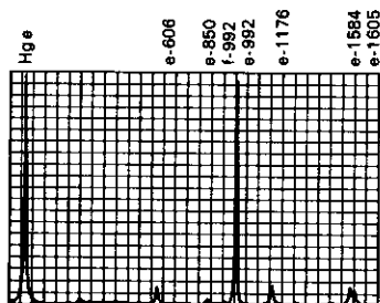
FIGURE 18.4 The spectrum of the Stokes radiation scattered by benzene. The line on the extreme left is the (greatly attenuated) exciting Hg \epsilon line at 22,938 \text{ cm}^{-1} ( 4358 \text{ \AA} ) that is the strongest line in the visible emission spectrum of Hg. The numbers on top give the downward shift in frequency (in \text{cm}^{-1} ), thus corresponding to the vibrational frequencies. They are preceded by letters indicating the parent Hg line. The f-992 line is due to the f line of Hg at 22,995 \text{ cm}^{-1} .
