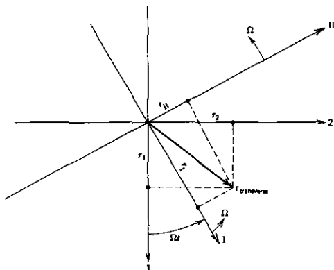
FIGURE 15.2 The relationship between the transverse components of \mathbf{r} in the {1, 2} and the rotating (I, II) coordinate system. System I, II, III rotates at a radian rate \Omega about the 3 axis (axes 3 and III coincide).
