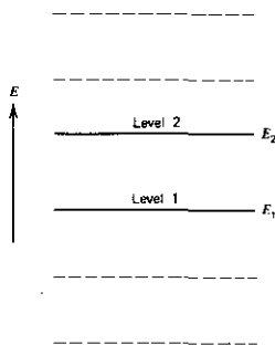
FIGURE 8.1 A two-level atomic system interacting with a radiation field whose frequency \omega is approximately equal to (E_2 - E_1)/\hbar . Other nonresonant levels (shown by broken lines) are assumed to play no role in the interaction except in determining the equilibrium populations N_{20} and N_{10} .
