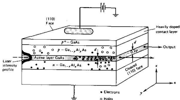
FIGURE 11.8 A typical double heterostructure GaAs-GaAlAs regions, respectively. Frequencies near \nu = E_g/\hbar are amplified by stimulating electron-hole recombination.
