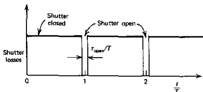
FIGURE 20.10 Periodic losses introduced by a shutter to induce mode locking. The presence of these losses favors the choice of mode phases that results in a pulse passing through the shutter during open intervals—that is, mode locking.
