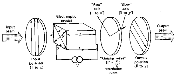
FIGURE 14.4 A typical electrooptic amplitude modulator. The total retardation \Gamma is the sum of the fixed retardation bias ( \Gamma_0 = \pi/2 ) introduced by the "quarter-wave" plate and that caused by the electrooptic crystal.
