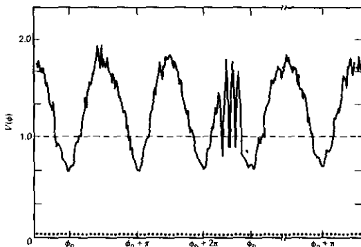
FIGURE 17.21 Measurement of the phase dependence of the quantum fluctuations in a squeezed state produced by parametric down conversion. The phase dependence of the rms noise voltage from a balanced homodyne detector is displayed as a function of local oscillator phase \phi at fixed analysis frequency (1.8 MHz) and bandwidth (100 KHz) in the spectral distribution of photocurrent fluctuations. With the optical parametric oscillator (OPO) blocked, the vacuum field entering the signal port of the detector produces the noise voltage given by the dashed line with no sensitivity on \phi . With the OPO input present, the dips below the vacuum level represent a 50% reduction in noise power relative to the vacuum noise level. Note that the ordinate is a linear scale in noise voltage. The dotted line is the amplifier noise level. (After Reference 32)
