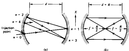
FIGURE 6.3 (a) Path of a ray injected in the plane of the figure into the space between two mirrors. (b) Reentrant ray in a symmetric confocal ( d = R ) mirror configuration repeating its pattern after two round trips.
