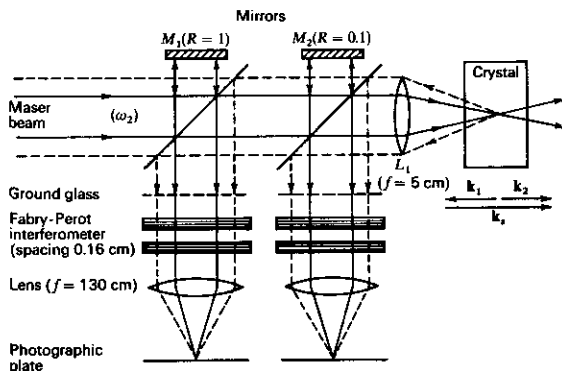
FIGURE 18.9 A schematic diagram of the experimental arrangement used to detect stimulated Brillouin scattering. The presence of a scattered optical beam at \omega_2 - \omega_1 is detected by the Fabry-Perot interferometer and causes additional "rings" to appear in the focal plane where they are photographed. Source: Reference 21.
