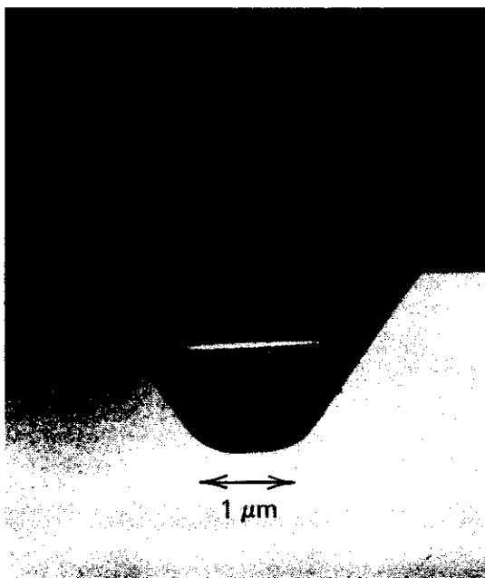
FIGURE 11.17 A buried crescent \text{InP}/\text{Ga}_{1-x}\text{In}_x\text{As}_{1-x}\text{P}_x/\text{InP} laser grown by a single-step liquid-phase epitaxy on an InP grooved substrate. Source: Courtesy of T.R. Chen, California Institute of Technology, Pasadena, Calif.
