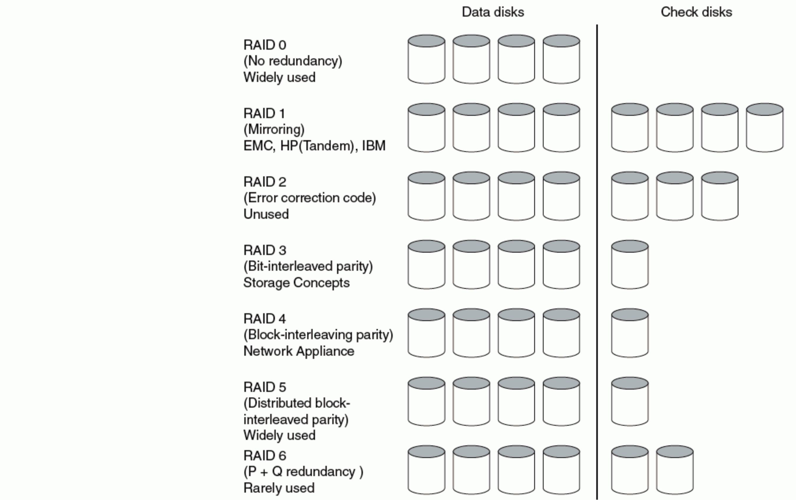
FIGURE 8.6 RAID for an example of four data disks showing extra check disks per RAID level and companies that use each level. Figures 8.7 and 8.8 explain the difference between RAID 3, RAID 4, and RAID 5.
