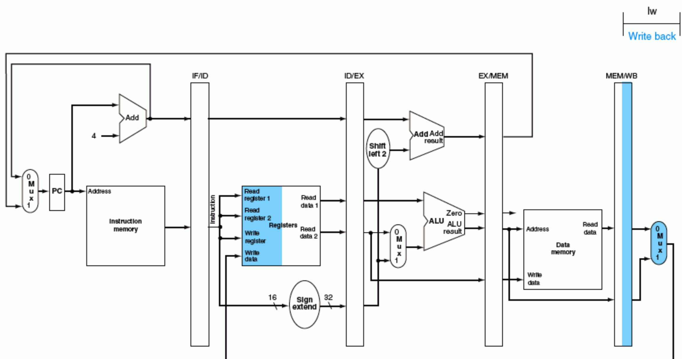
FIGURE 6.14 MEM and WB: the fourth and fifth pipe stages of a load instruction, highlighting the portions of the datapath in Figure 6.11 used in this pipe stage. Data memory is read using the address in the EX/MEM pipeline registers, and the data is placed in the MEM/WB pipeline register. Next, data is read from the MEM/WB pipeline register and written into the register file in the middle of the datapath.
