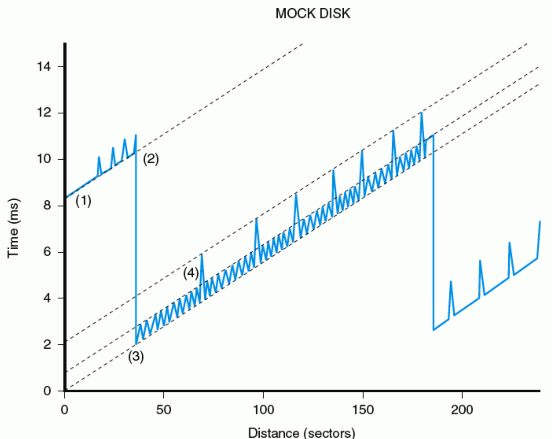
FIGURE 8.17 Example output of Skippy for a hypothetical disk.
