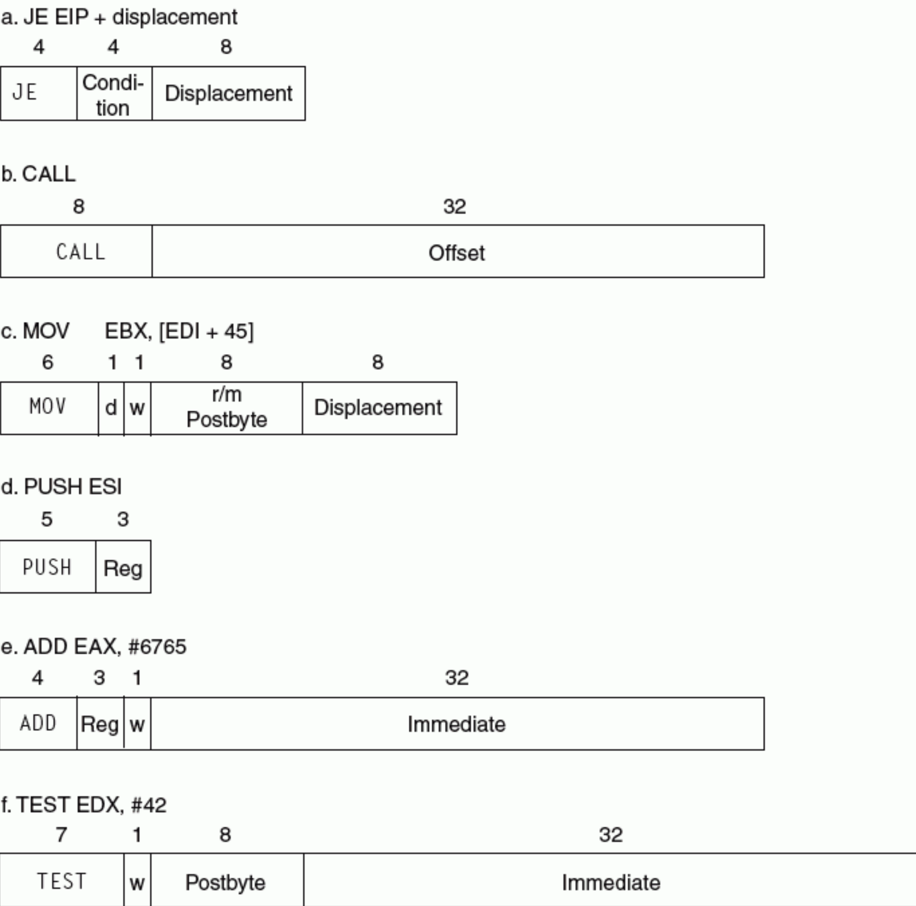
FIGURE 2.45 Typical IA-32 instruction formats. Figure 2.46 shows the encoding of the postbyte. Many instructions contain the 1-bit field w, which says whether the operation is a byte or double word. The d field in MOV is used in instructions that may move to or from memory and shows the direction of the move. The ADD instruction requires 32 bits for the immediate field because in 32-bit mode the immediates are either 8 bits or 32 bits. The immediate field in the TEST is 32 bits long because there is no 8-bit immediate for test in 32-bit mode. Overall, instructions may vary from 1 to 17 bytes in length. The long length comes from extra 1-byte prefixes, having both a 4-byte immediate and a 4-byte displacement address, using an opcode of 2 bytes, and using the scaled index mode specifier, which adds another byte.
