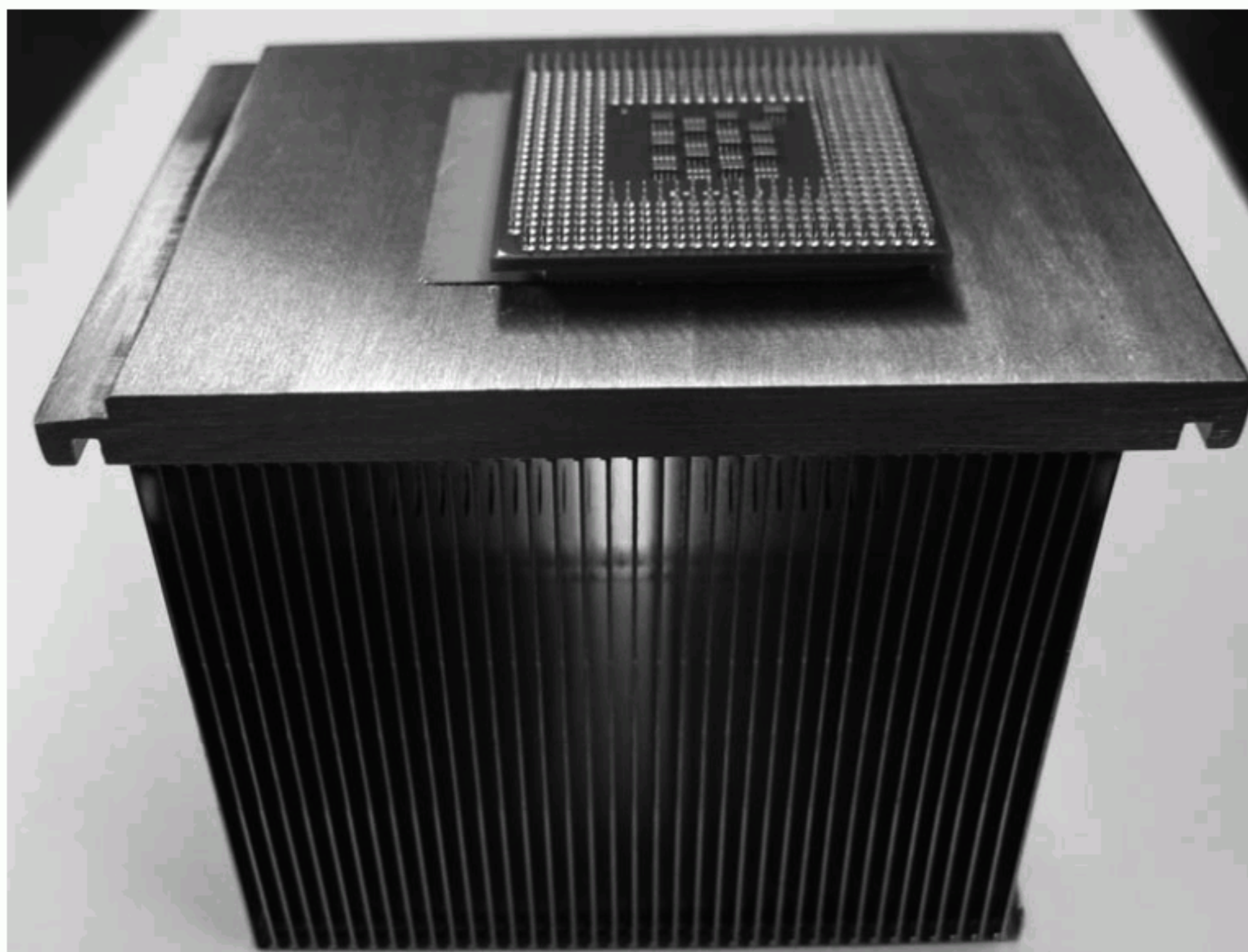
FIGURE 1.16 An Intel Pentium 4 (3.06 GHz) mounted on top of its heat sink, which is designed to remove the 82 watts generated within the die.
