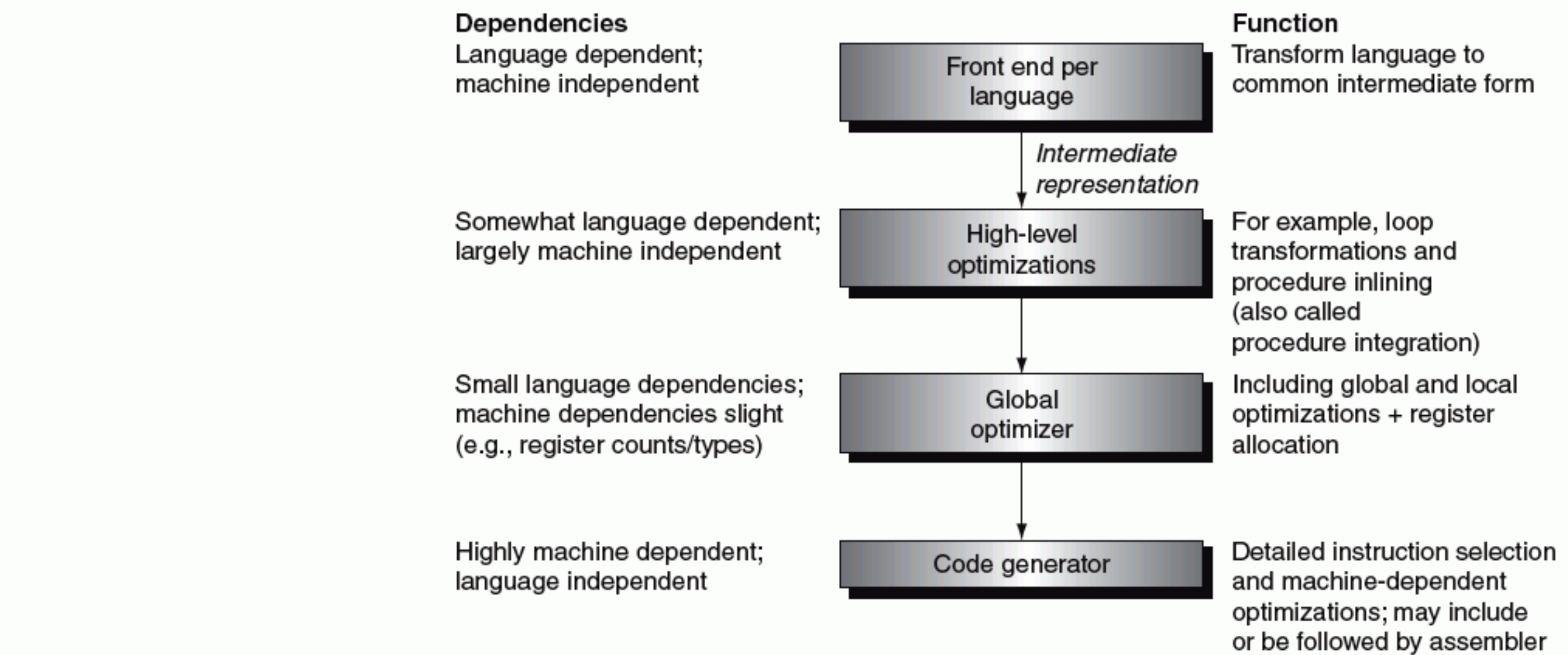
FIGURE 2.31 The structure of a modern optimizing compiler consists of a numbers of passes or phases. Logically each pass can be thought of as running to completion before the next occurs. In practice, some passes may handle a procedure at a time, essentially interleaving with another pass.
