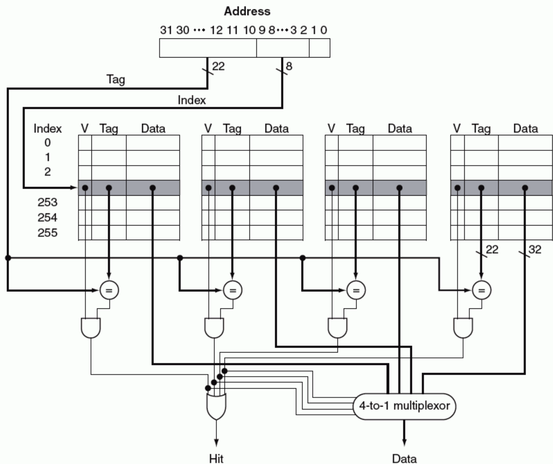
FIGURE 7.17 The implementation of a four-way set-associative cache requires four comparators and a 4-to-1 multiplexor. The comparators determine which element of the selected set (if any) matches the tag. The output of the comparators is used to select the data from one of the four blocks of the indexed set, using a multiplexor with a decoded select signal. In some implementations, the Output enable signals on the data portions of the cache RAMs can be used to select the entry in the set that drives the output. The Output enable signal comes from the comparators, causing the element that matches to drive the data outputs. This organization eliminates the need for the multiplexor.
