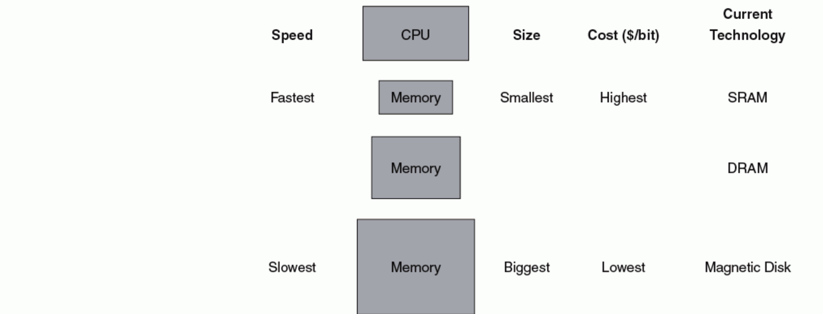
FIGURE 7.1 The basic structure of a memory hierarchy. By implementing the memory system as a hierarchy, the user has the illusion of a memory that is as large as the largest level of the hierarchy, but can be accessed as if it were all built from the fastest memory.
