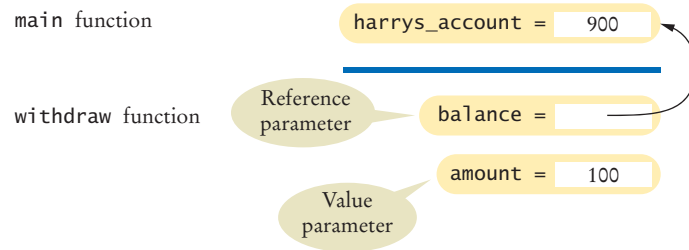
Figure 7 Reference and Value Parameters
