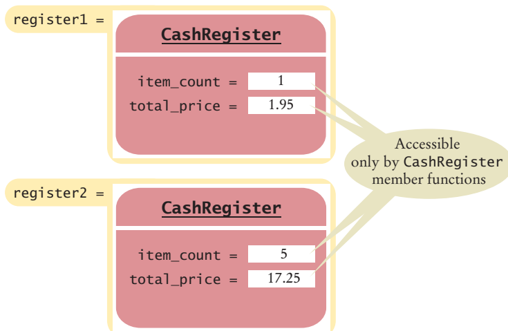
Figure 2 Data Members of CashRegister Objects
