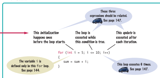
You can visualize the for loop as an orderly sequence of steps.
