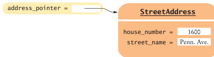
Figure 11 A Pointer to a Structure
