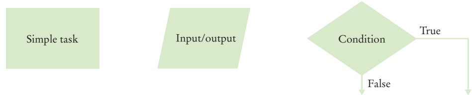
Figure 5 Flowchart Elements
