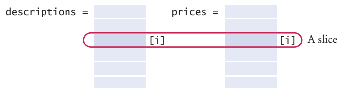
Figure 5 Parallel Vectors
