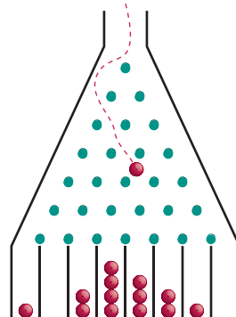
Figure 9 A Galton Board
