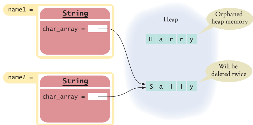
Figure 10 A Bad Assignment
