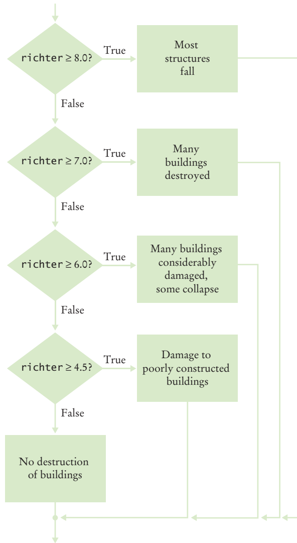
Figure 3 Multiple Alternatives
