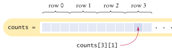
Figure 13 A Two-Dimensional Array is Stored as a Sequence of Rows
