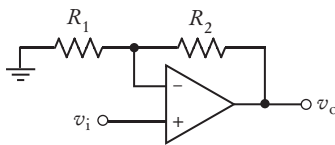
(a) Amplifier
