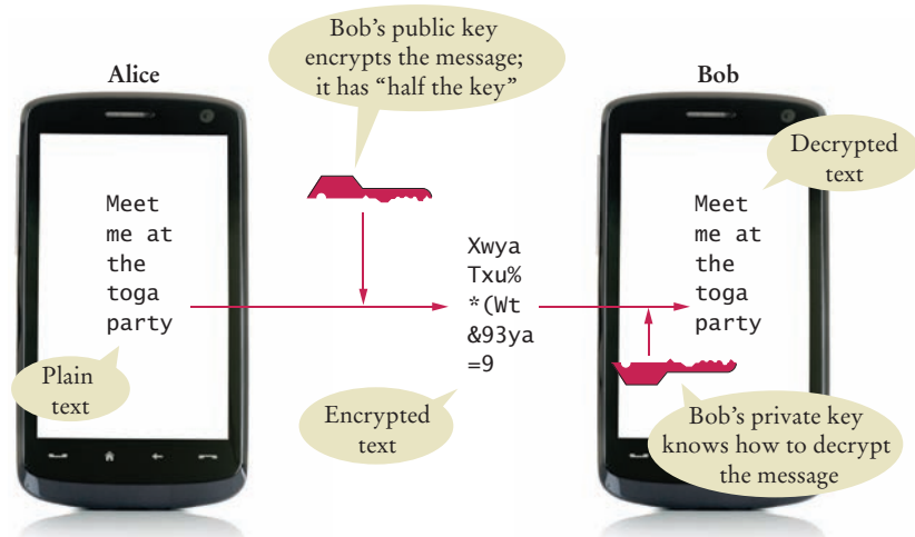
Public-Key Encryption
