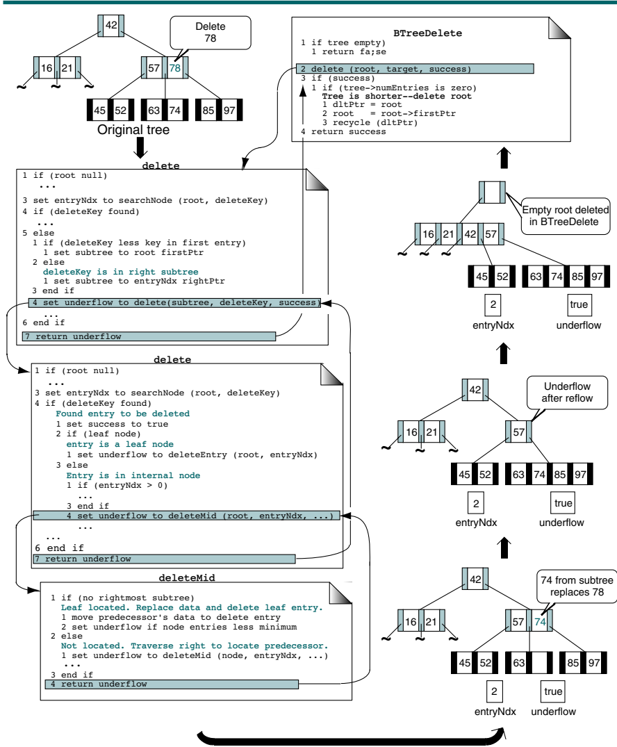
FIGURE 10-11 B-tree Deletions
