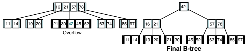
FIGURE 10-9 Building a B-tree of Order 5
