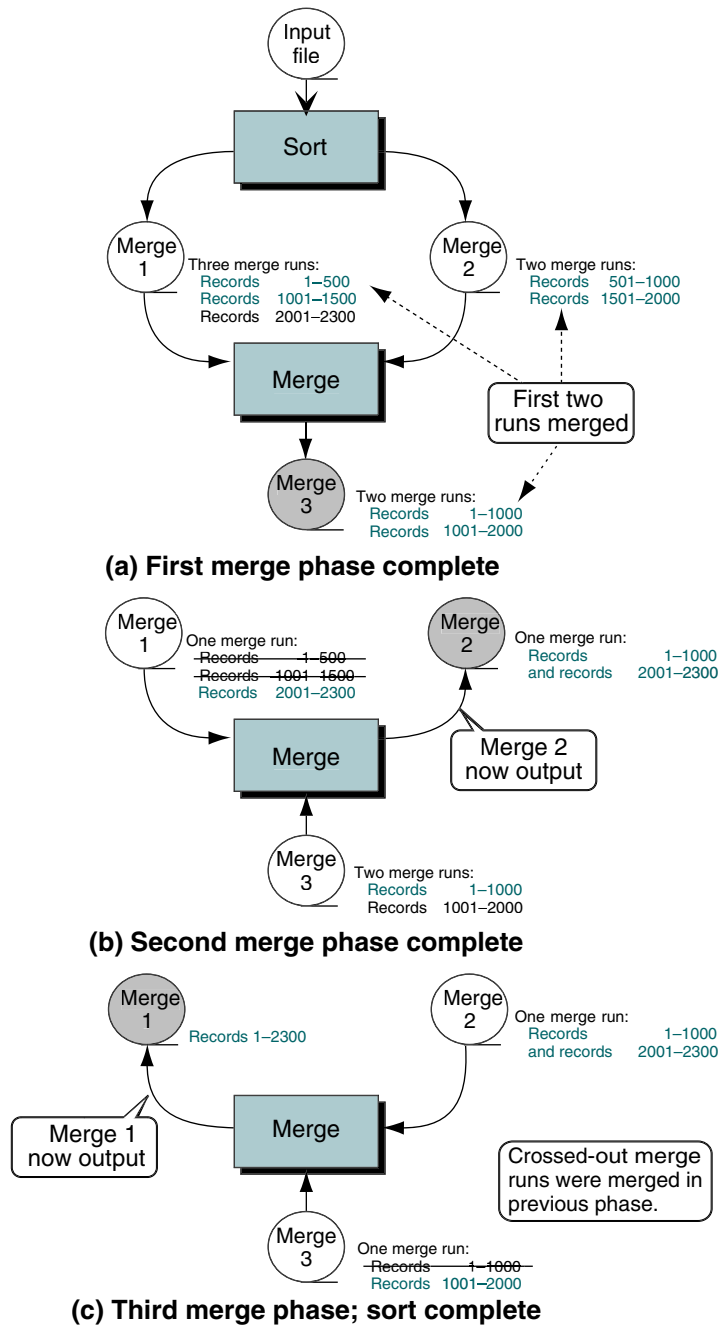
FIGURE 12-22 Polyphase Merge Sort
