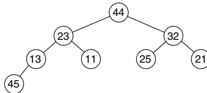
FIGURE 9-19 Nonheap Structure for Exercise 3
