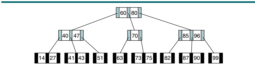
FIGURE 10-24 B-tree for Exercises 10 and 11
