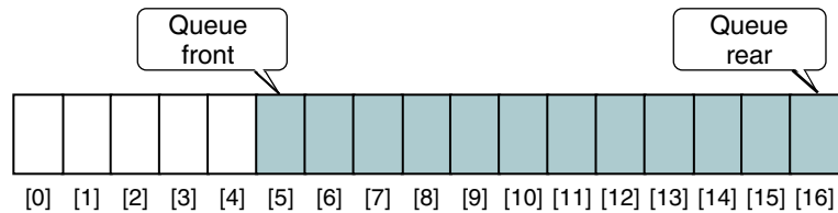
FIGURE F-3 Array Queue with Last Element Filled
