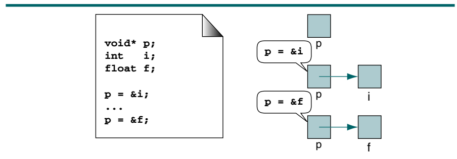
FIGURE 1-7 Pointers for Program 1-1
