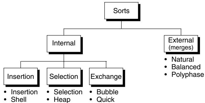
FIGURE 12-1 Sort Classifications
