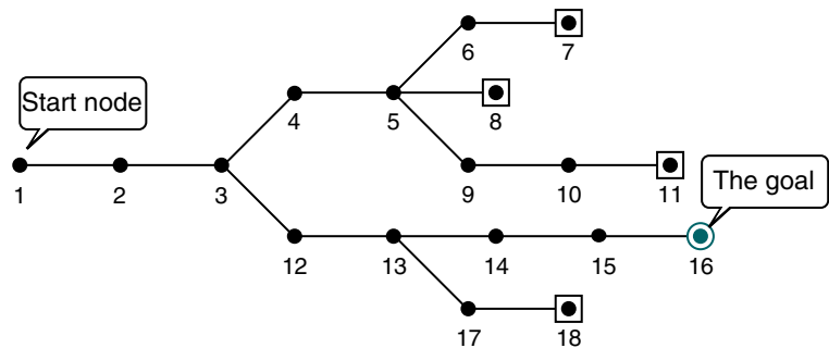
FIGURE 3-17 Backtracking Example
