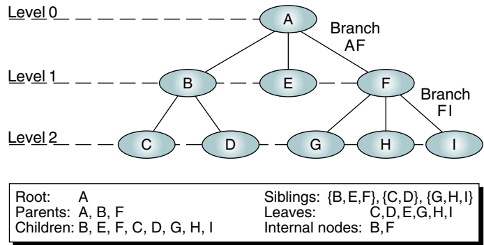
FIGURE 6-2 Tree Nomenclature
