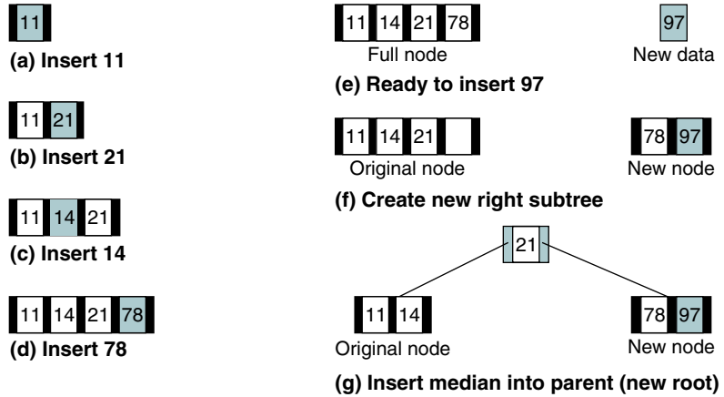
FIGURE 10-5 B-tree Insert Overview
