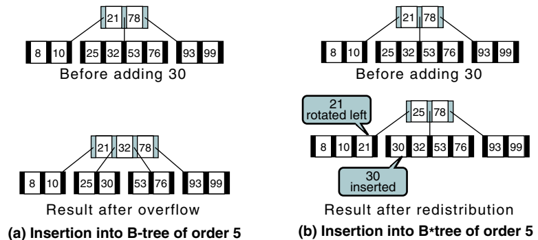
FIGURE 10-20 B*tree Insertion
