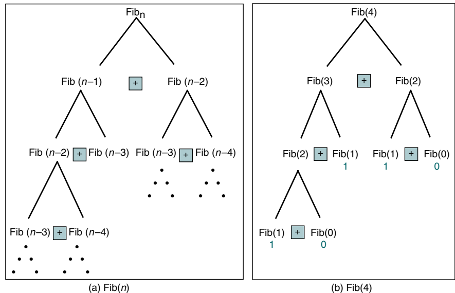
FIGURE 2-8 Fibonacci Numbers
