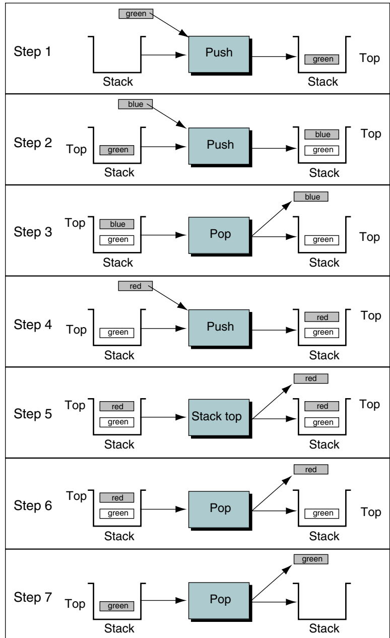
FIGURE 3-5 Stack Example
