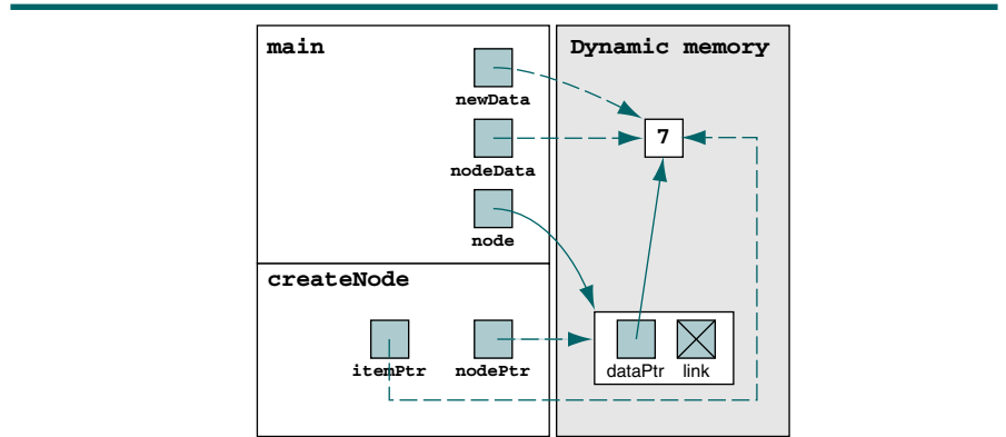
FIGURE 1-9 Pointers for Programs 1-2 and 1-3
