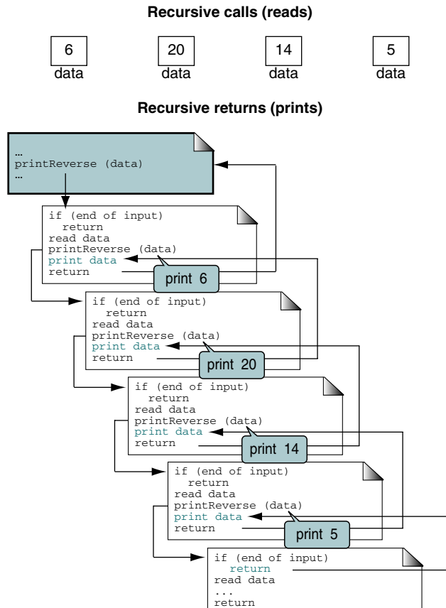
FIGURE 2-5 Print Keyboard Input in Reverse
